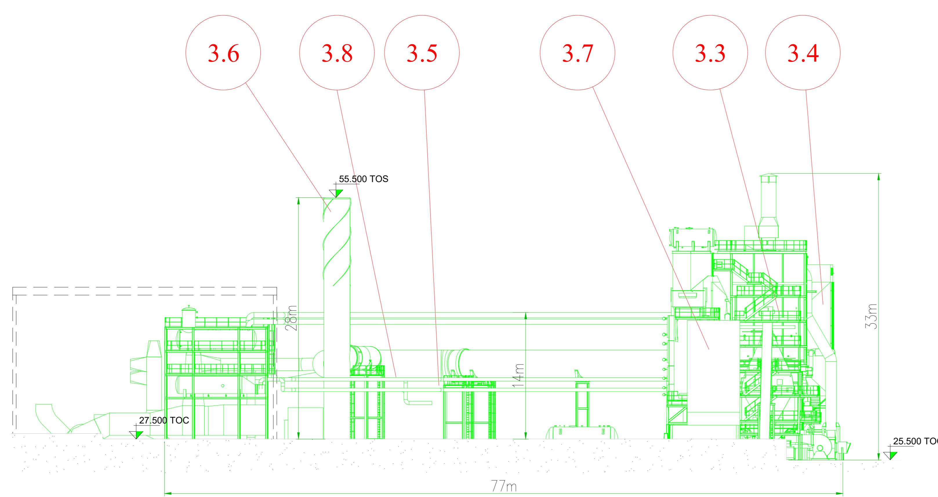
Section C-C
